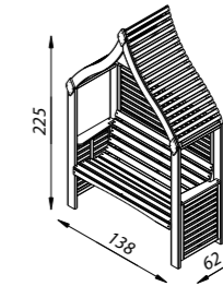
040205 138 x 62 x 225 SIENA OPEN VIEW
